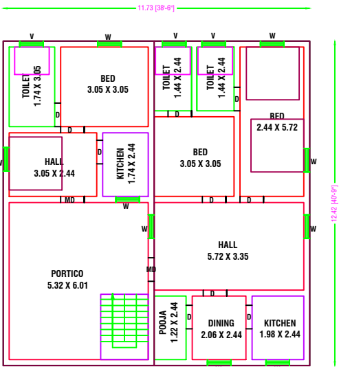
PRO. GROUND FLOOR PLAN [SOUTH FACING]
