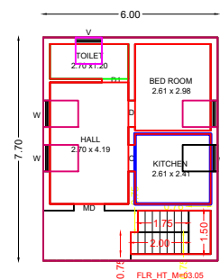
GROUND FLOOR PLAN SOUTH FACING
