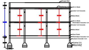
Section Section - AA
