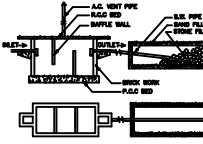
SEPTIC TANK DETAILS
