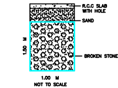
RAIN WATER HARVEST COLLECTION PIT.
