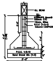
R.C.C. COLUMN FOOTING DETAILS
