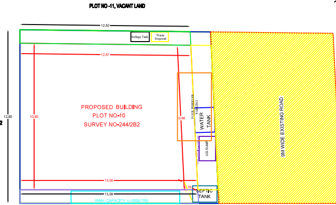
PROPOSED BUILDING PLOT NO-10 SURVEY NO-244/2B2 SITE PLAN
