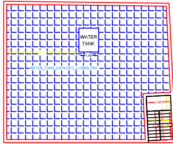
TERRACE PLAN
