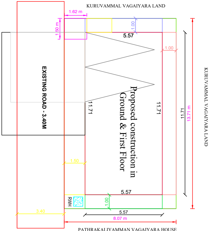
SITE PLAN
