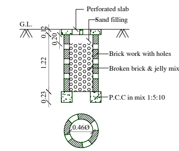
PERCOLATION PTT
