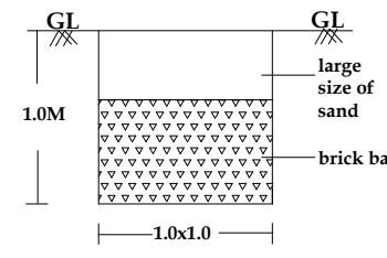
RAINWATER HARVESTING
