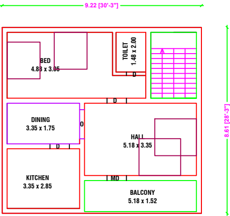
PRO.FIRST FLOOR PLAN EAST FACING
