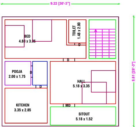
PRO.GROUND FLOOR PLAN EAST FACING
