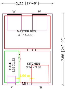
GROUND FLOOR PLAN ( EAST FACING )
