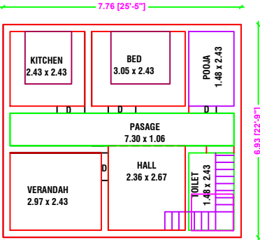
PRO.FIRST FLOOR PLAN NORTH FACING
