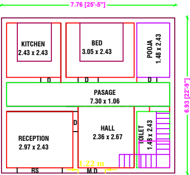
EX.GROUND FLOOR PLAN NORTH FACING
