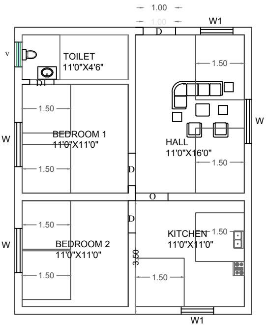
PROPOSED GROUND FLOOR PLAN (NORTH FACING)
