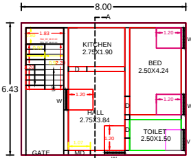
GROUND FLOOR PLAN (Facing North)
