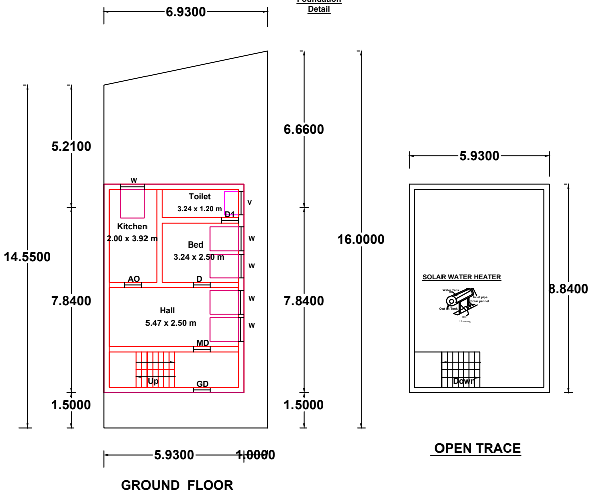
GROUND FLOOR
