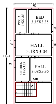
EXIST GROUND FLOOR PLAN
