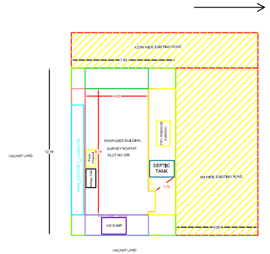
SITE PLAN
