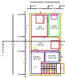
PROPOSED GROUND FLOOR PLAN
