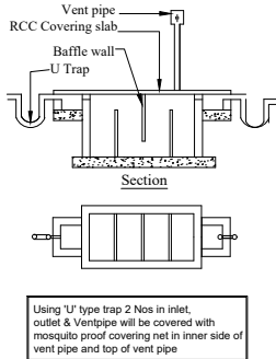
Septic Tank With trap Not To Scale
