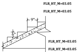
Staircase Detail Not To Scale
