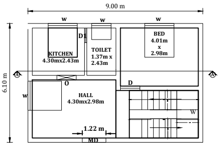
GROUND FLOOR PLAN ( FACING NORTH )
