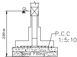
Isolated Footing -A (1.50X1.50) (Not to Scale) FOUNDATION DETAIL - A
