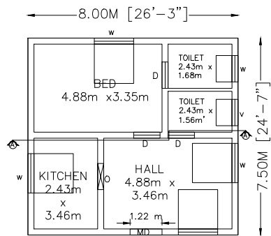
GROUND FLOOR PLAN ( FACING WEST )
