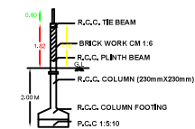
COMPOUND WALL DETAILS
