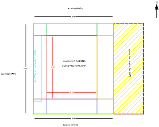
SITE PLAN
