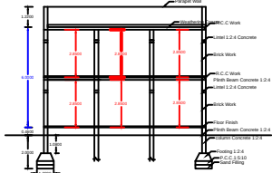
SECTION SECTION - AB
