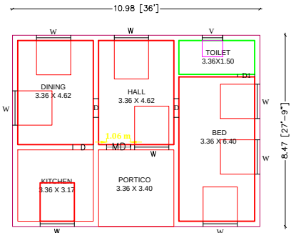
GROUND FLOOR PLAN EAST FACING
