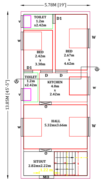
GROUND FLOOR PLAN SOUTH FACING )
