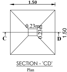
SECTION - 'CD'
