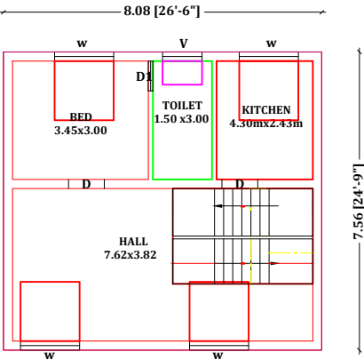
FIRST FLOOR PLAN ( FACING WEST )
