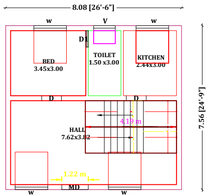
GROUND FLOOR PLAN ( FACING WEST )
