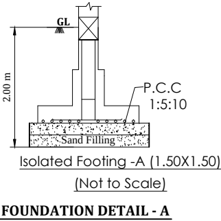
FOUNDATION DETAIL - A
