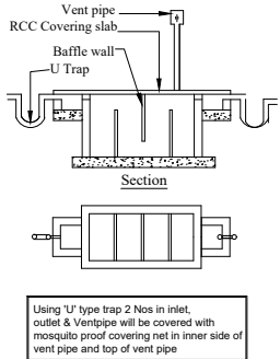
Septic Tank With Not To Scale
