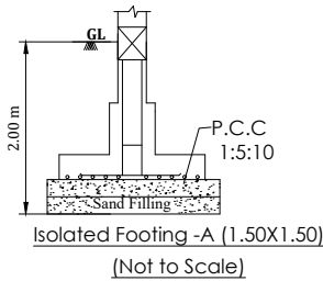
FOUNDATION DETAIL - A
