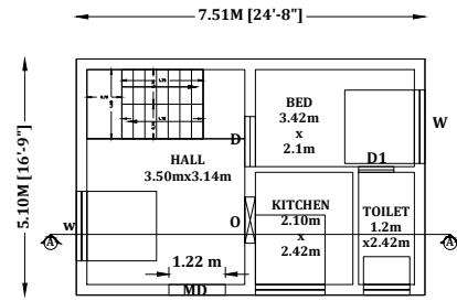
GROUND FLOOR PLAN (SOUTH FACING )
