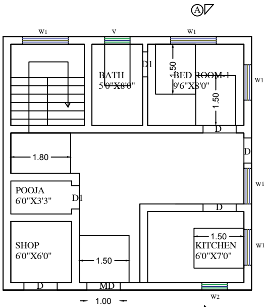
PROPOSED GROUND FLOOR PLAN (SOUTH FACING)
