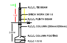
COMPOUND WALL DETAILS
