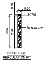
DETAILS OF PERCOLATION PIT
