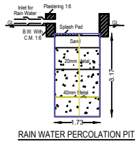
RAIN WATER PERCOLATION PIT
