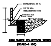
RAIN WATER COLLECTION TRENCH (SCALE-1:100)
