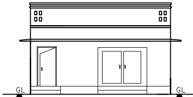
FRONT ELEVATION
