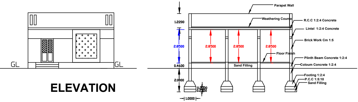
Section Section - AA
