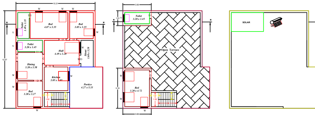
Exist Ground Floor Plan South facing
