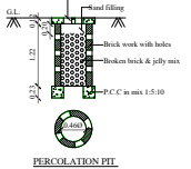
PERCOLATION PIT
