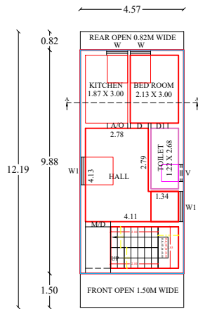
GROUND FLOOR PLAN (NORTH FACING)
