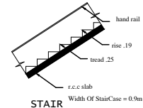
STAIR
