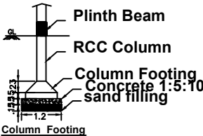
Foundation Detail
