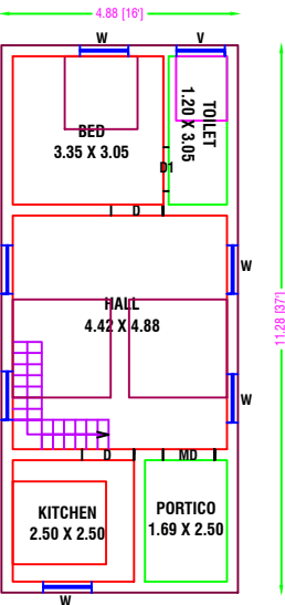
PRO. GROUND FLOOR EAST FACING
