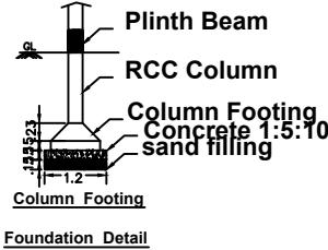
Foundation Detail
