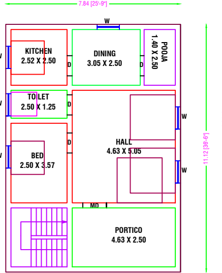
PRO. GROUND FLOOR
