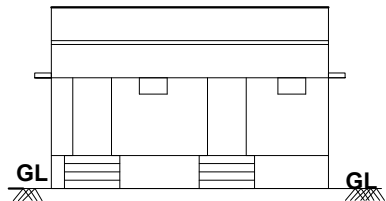
FRONT ELEVATION
