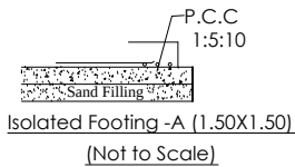
FOUNDATION DETAIL - A
