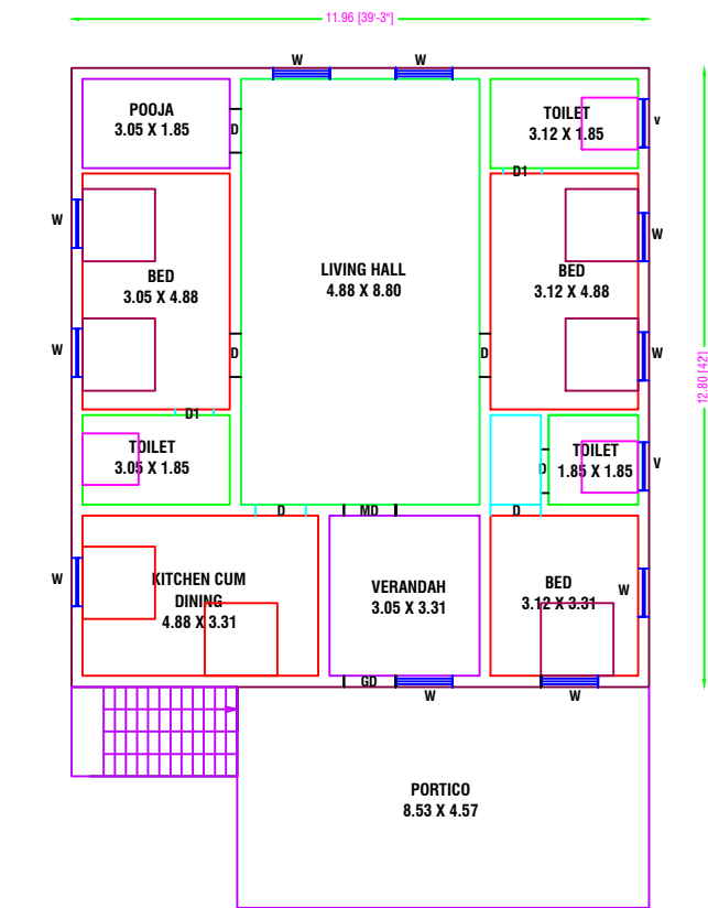
PRO. GROUND FLOOR [EAST FACING]
