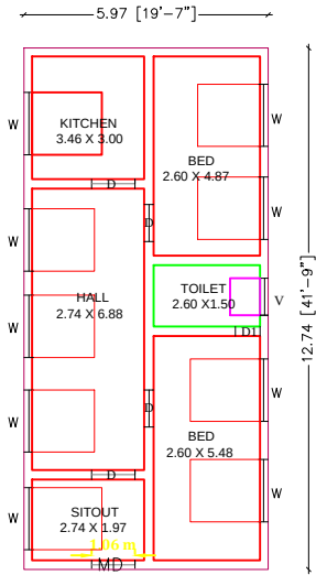
GROUND FLOOR PLAN NORTH FACING
