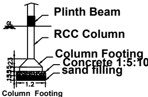
Foundation Detail
