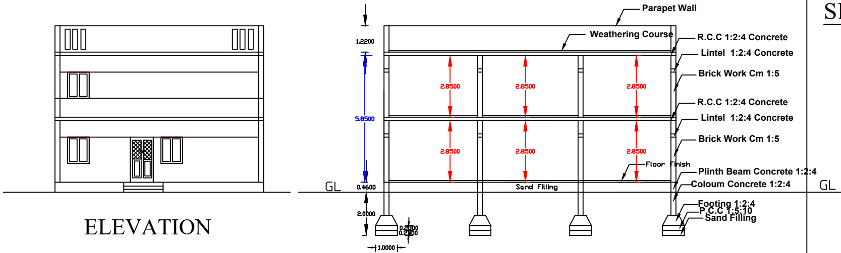
Section - AA
