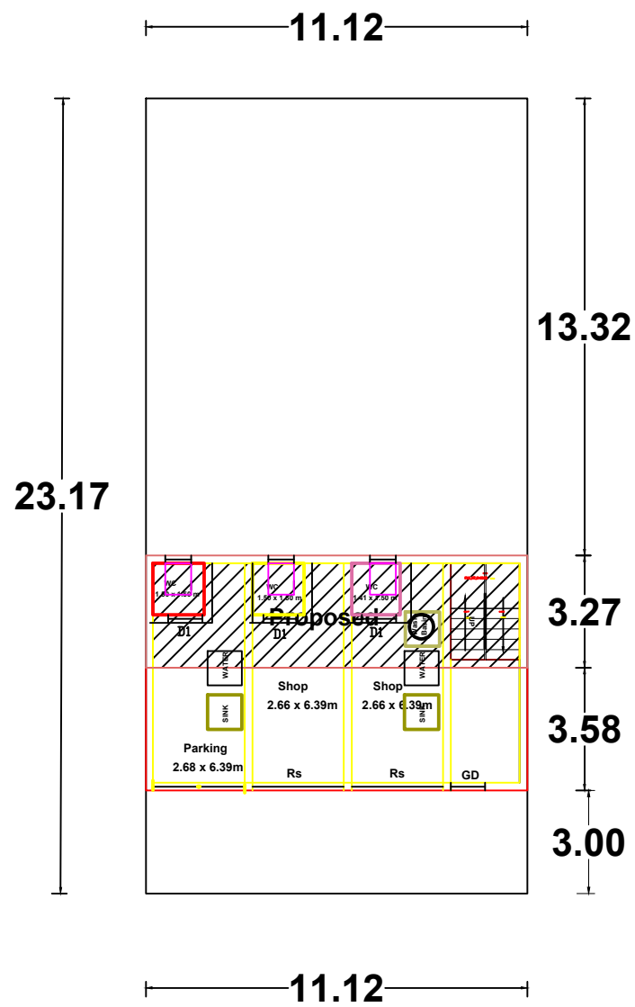
GROUND FLOOR PLAN (EXISTING - COMMERCIAL) AND PROPOSED GROUND FLOOR PLAN
