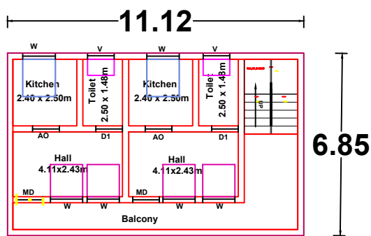
FIRST FLOOR PLAN ( PROPOSED )
