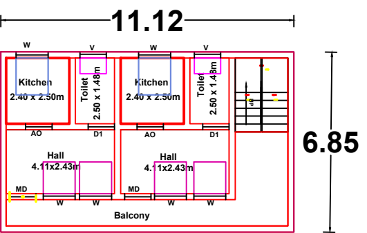
SECOND FLOOR PLAN ( PROPOSED )
