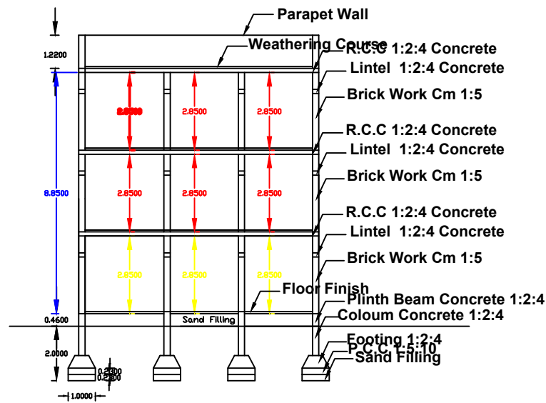
Section Section - AA
