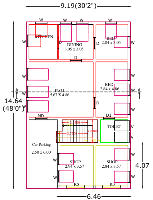
GROUND FLOOR PLAN (NORTH FACING)
