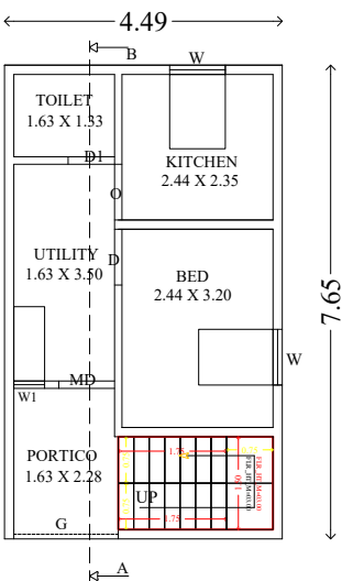
EXISTING GROUND FLOOR
