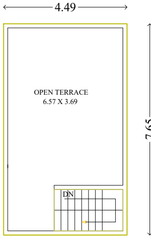
PROPOSED TERRACE FLOOR
