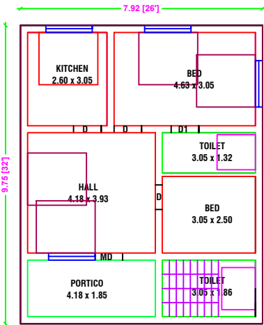
PRO.GROUND FLOOR PLAN NORTH FACING
