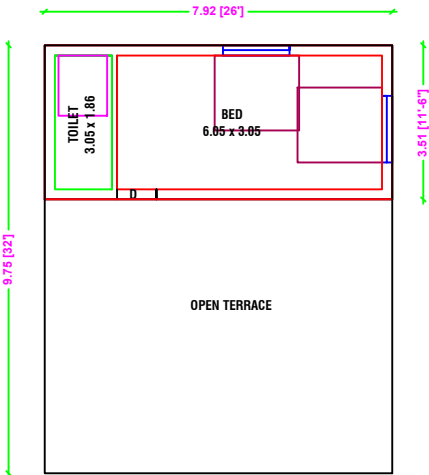
PRO.FIRST FLOOR PLAN NORTH FACING
