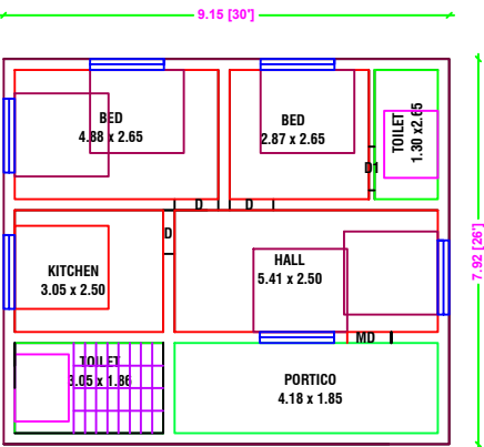
PRO.GROUND FLOOR PLAN EASTFACING
