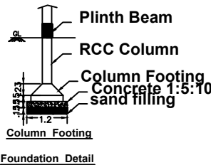
Foundation Detail
