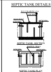
SEPTIC TANK PLAN
