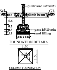
COLUMN FOUNDATION
