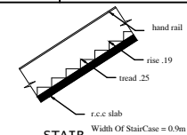
STAIR Width Of StairCase = 0.9m
