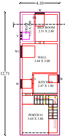
GROUND FLOOR PLAN (EXISTING BUILDING) (SOUTH FACING)
