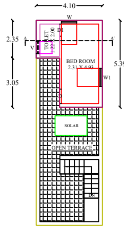
SECOND FLOOR PLAN (PROPOSED BUILDING)
