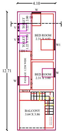
FIRST FLOOR PLAN (EXISTING BUILDING)
