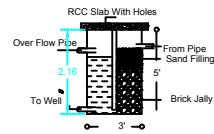
RWHS Tank Details
