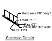
Staircase Details
