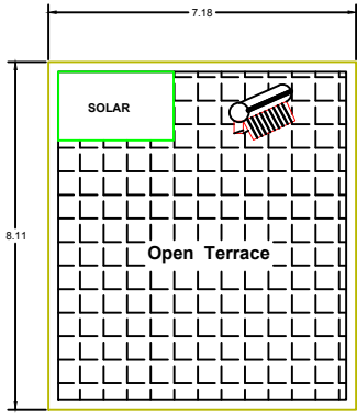
Proposed Terrace Floor Plan
