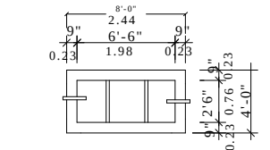
PLAN SEPTIC TANK DETAIL
