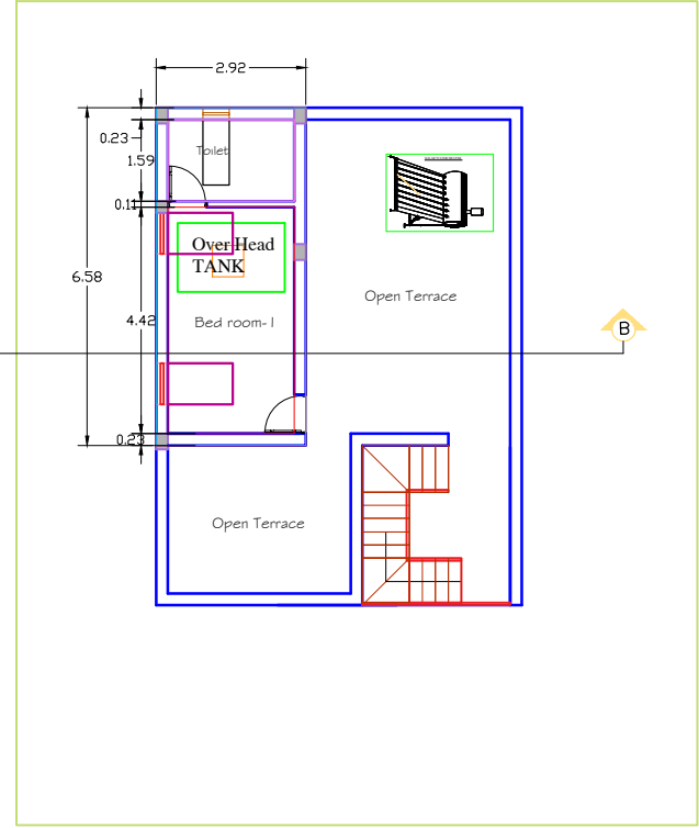
FIRST/ TERRACE FLOOR PLAN BLOC .1
