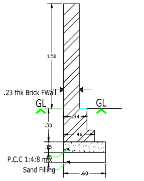
Compound Wall Section detail
