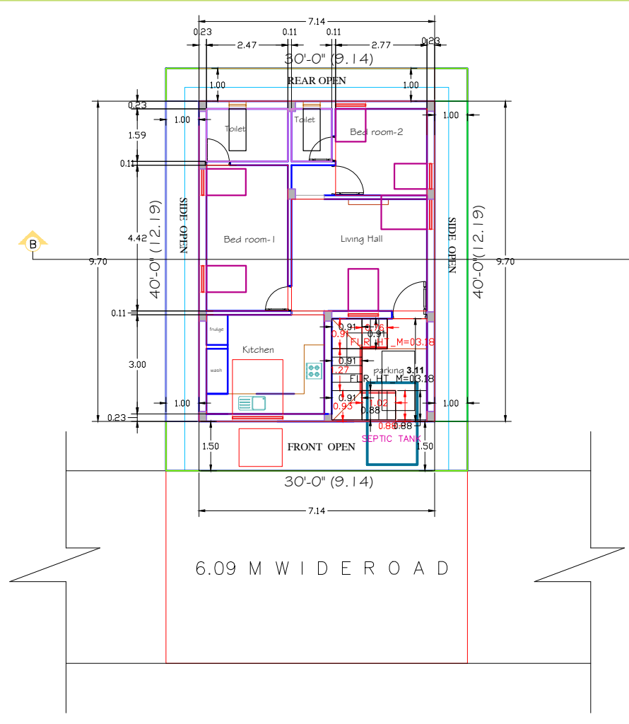
SITE/ PROPOSED GROUND FLOOR PLAN BLOC .1
