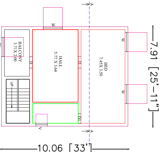
FIRST FLOOR PLAN (NORTH FACING)
