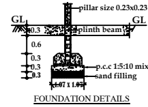
FOUNDATION DETAILS
