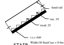
STAIR
